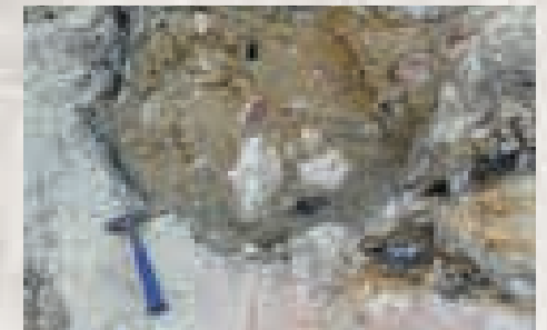
Bunte Breccia from the Harburg-Ronheim quarry.
