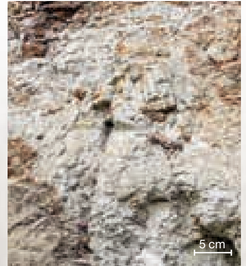
Rocks of the crystalline basement strongly changed ("shocked") by the impact.
