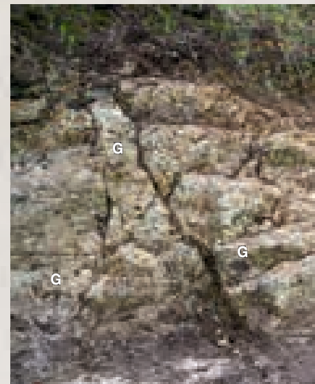
The former Suevite quarry at Doosweiher shows the rock in a slightly weathered state. Gray, protruding, bulbous structures are small “Flädle” (G – re-solidified molten rock).
